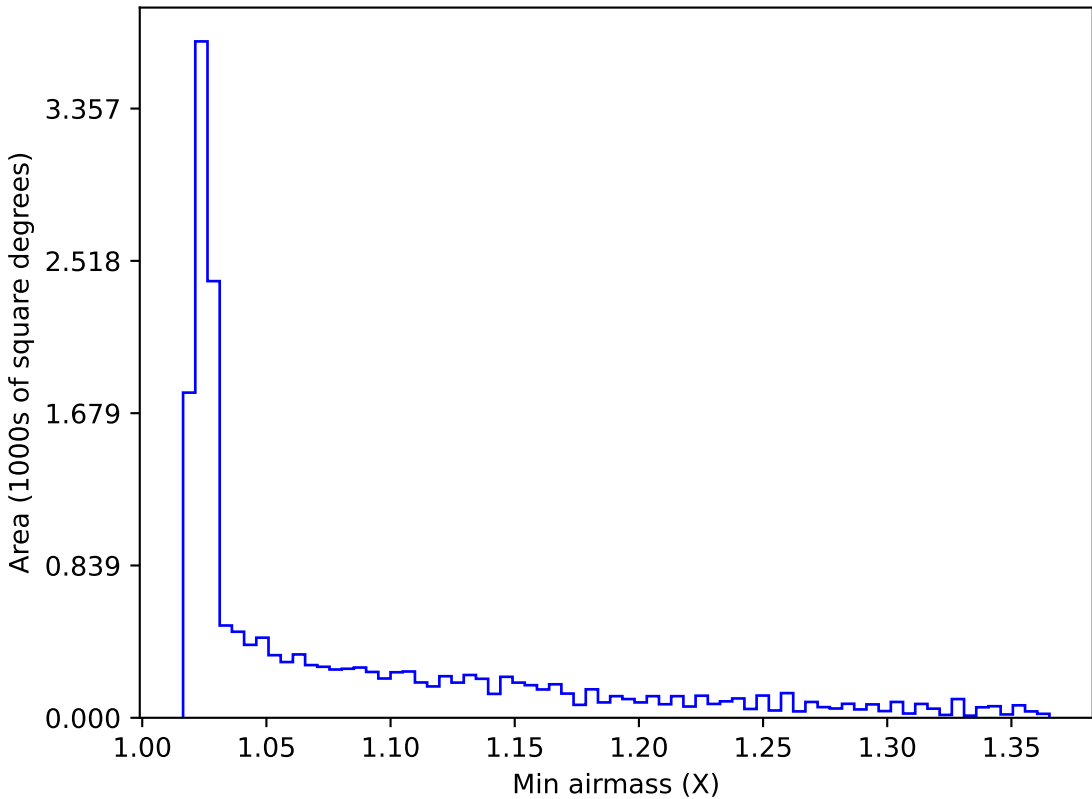
roll_pause_mjdp60_v3.4_10yrs WFD all bands: Min airmass
