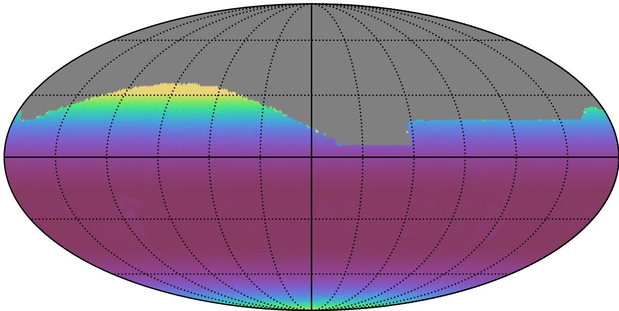
roll_pause_mjdp60_v3.4_10yrs All sky z band: Min airmass
