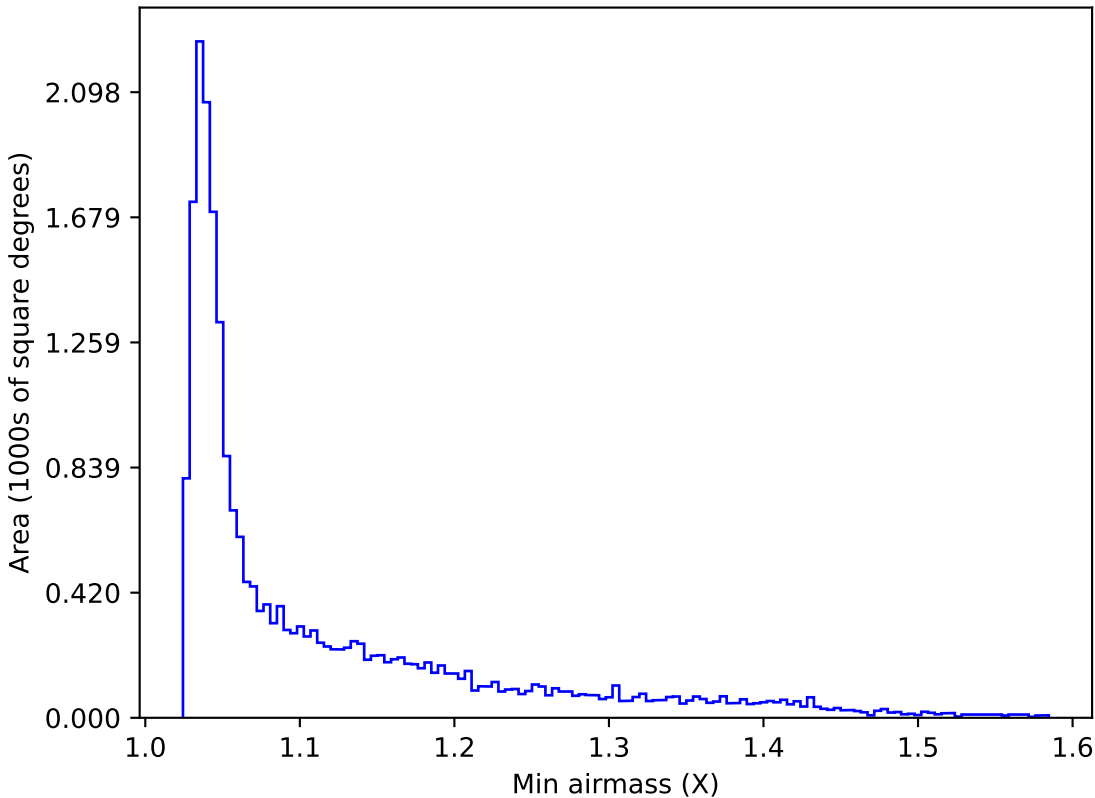
roll_pause_mjdp60_v3.4_10yrs All sky u band: Min airmass
