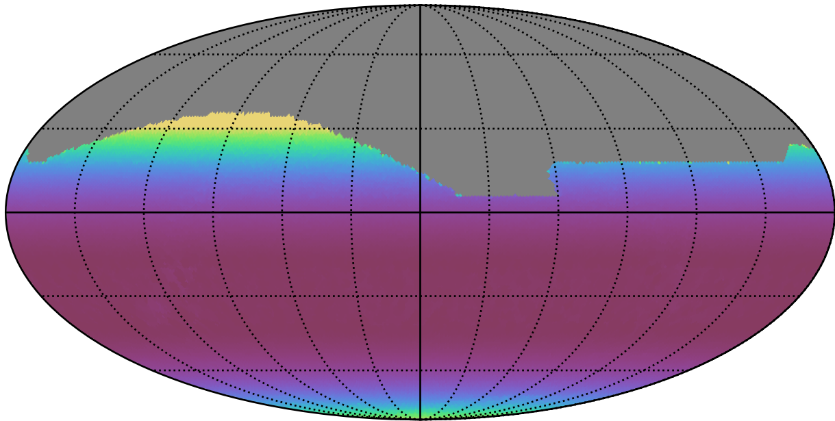
roll_pause_mjdp60_v3.4_10yrs All sky i band: Min airmass
