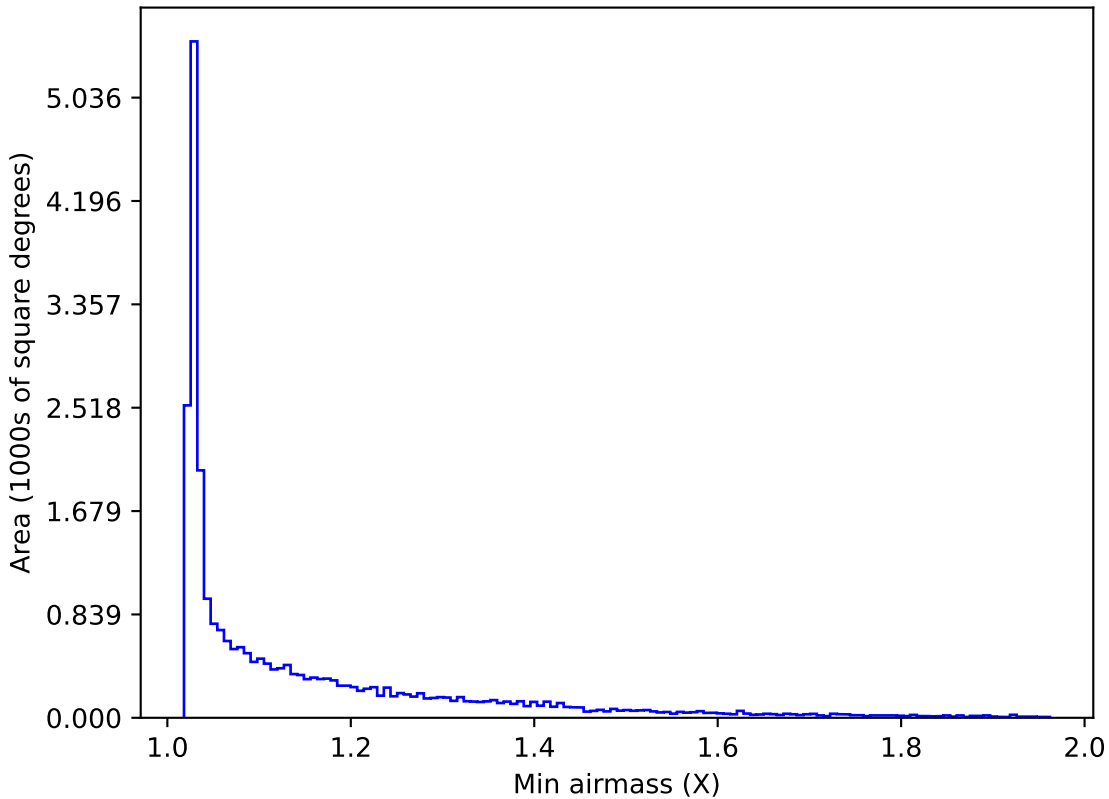
roll_pause_mjdp60_v3.4_10yrs All sky i band: Min airmass
