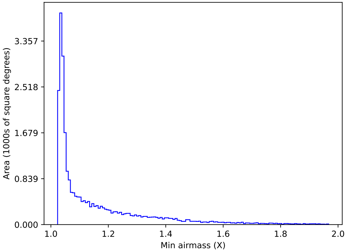
roll_pause_mjdp60_v3.4_10yrs All sky g band: Min airmass
