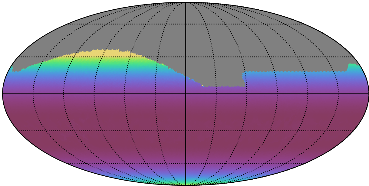
roll_pause_mjdp60_v3.4_10yrs All sky all bands: Min airmass
