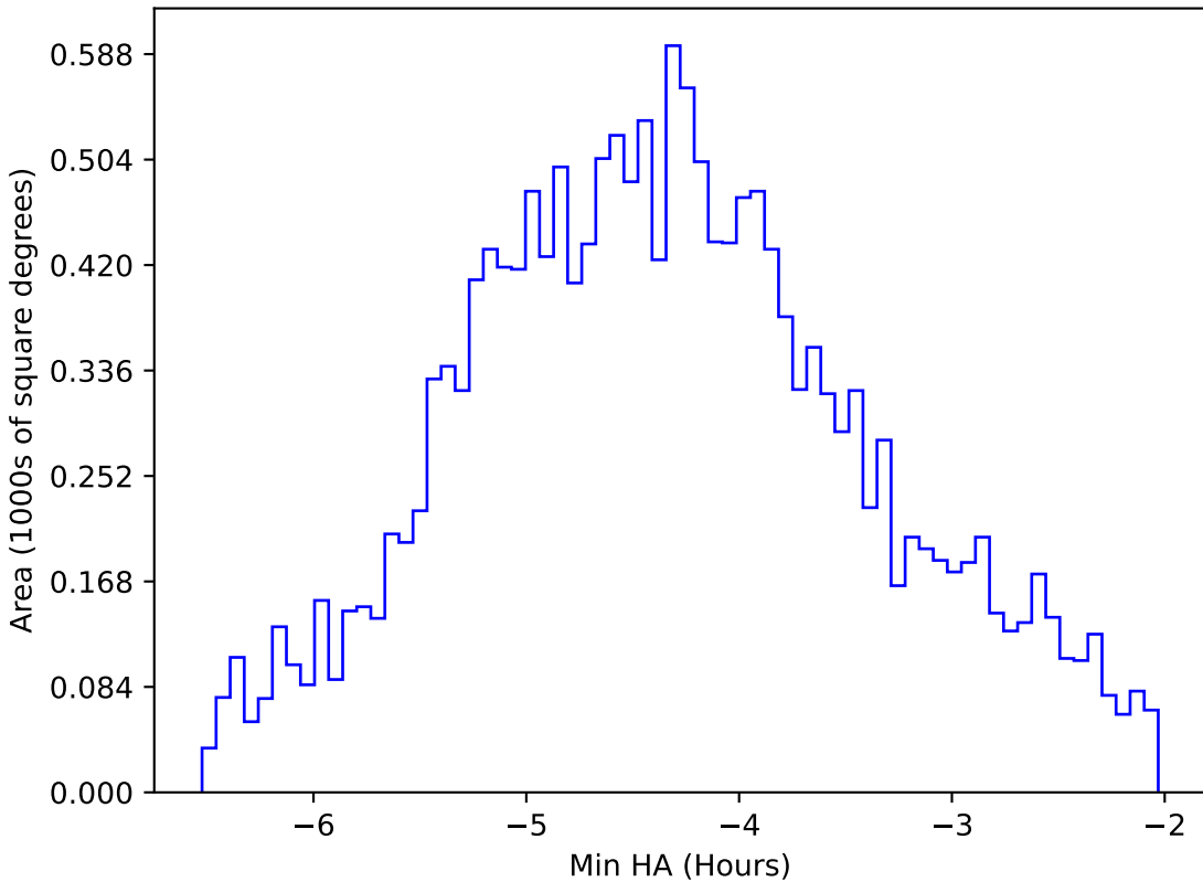
roll_pause_mjdp60_v3.4_10yrs WFD z band: Min HA
