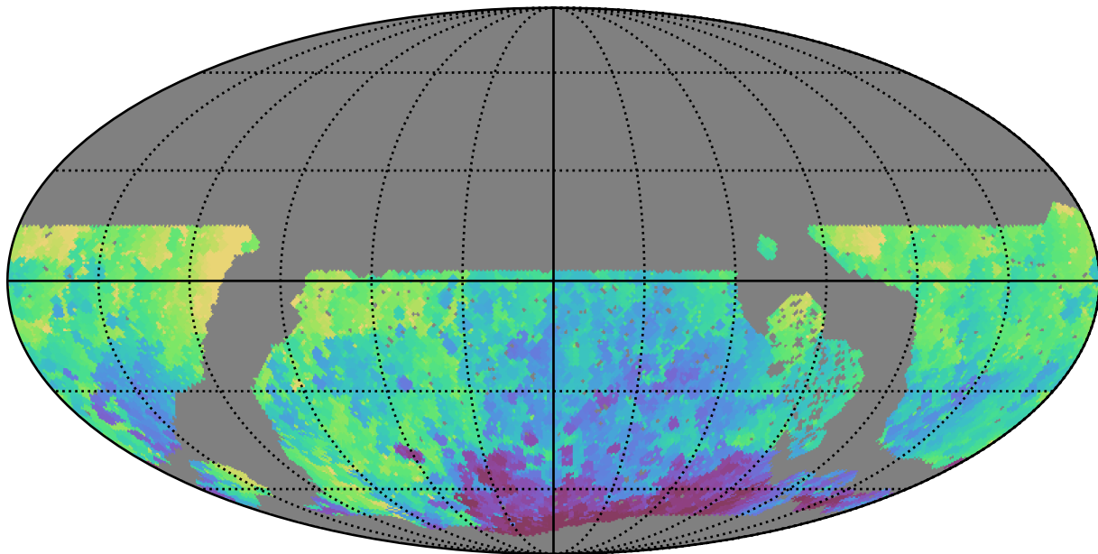
roll_pause_mjdp60_v3.4_10yrs WFD y band: Min HA
