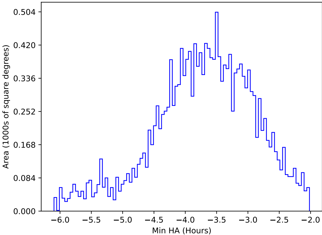
roll_pause_mjdp60_v3.4_10yrs WFD y band: Min HA
