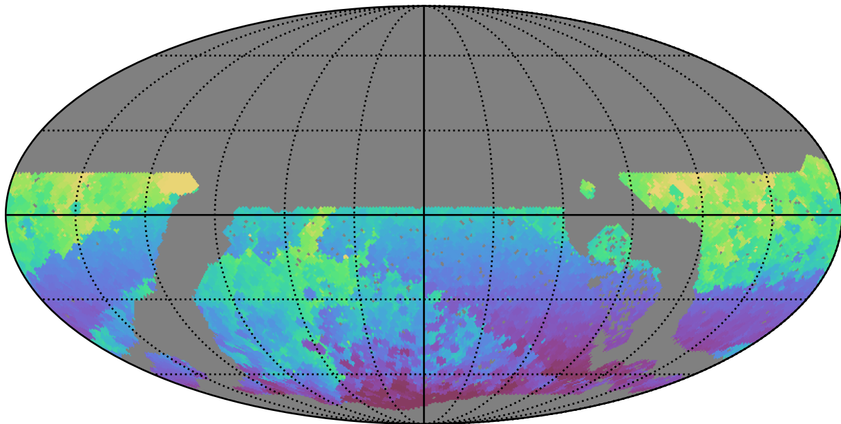
roll_pause_mjdp60_v3.4_10yrs WFD r band: Min HA
