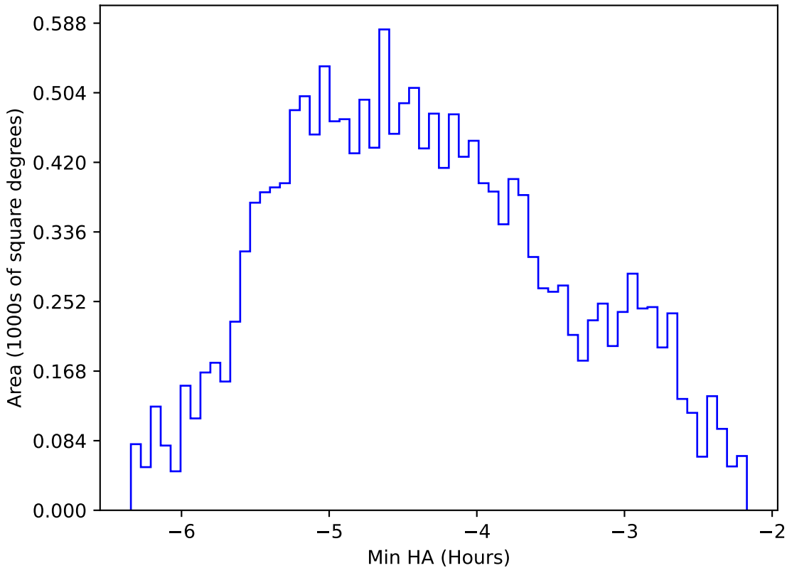
roll_pause_mjdp60_v3.4_10yrs WFD r band: Min HA
