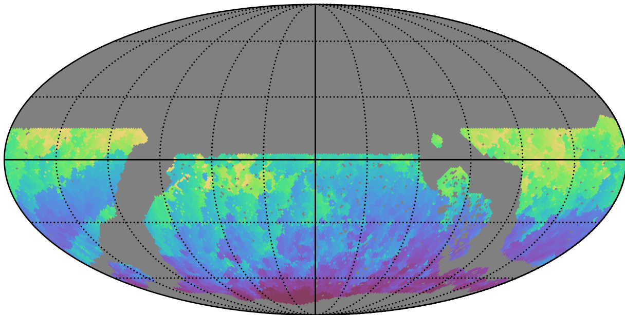
roll_pause_mjdp60_v3.4_10yrs WFD i band: Min HA
