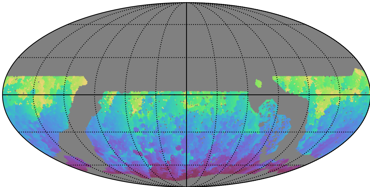
roll_pause_mjdp60_v3.4_10yrs WFD g band: Min HA
