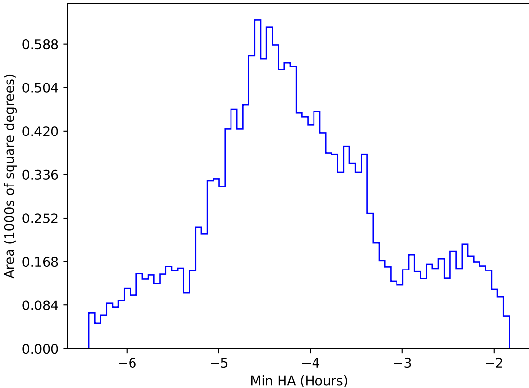
roll_pause_mjdp60_v3.4_10yrs WFD g band: Min HA
