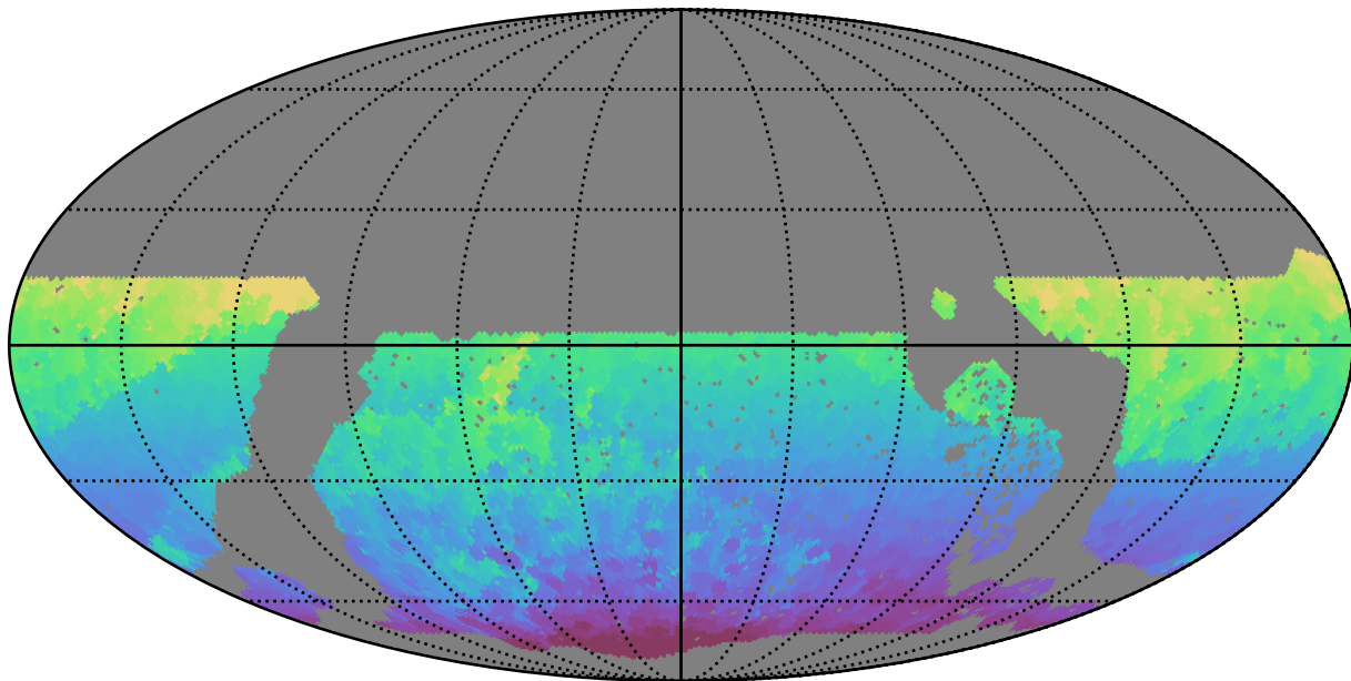
roll_pause_mjdp60_v3.4_10yrs WFD all bands: Min HA
