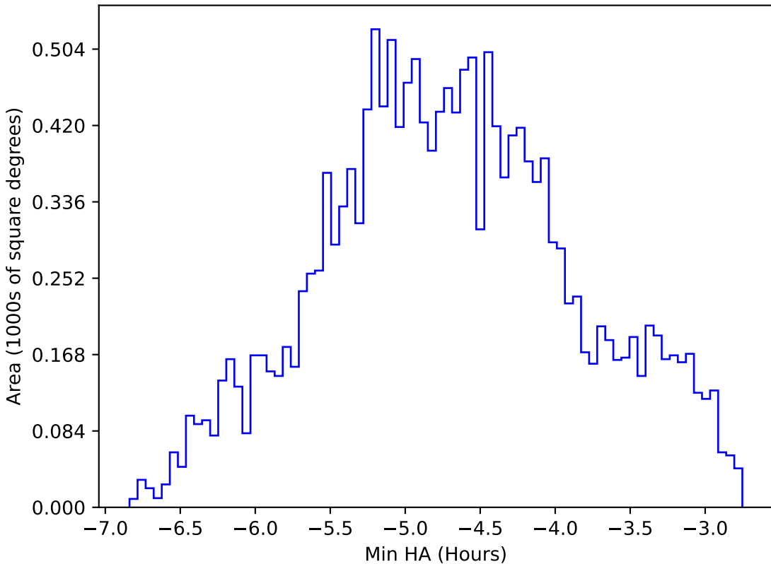
roll_pause_mjdp60_v3.4_10yrs WFD all bands: Min HA
