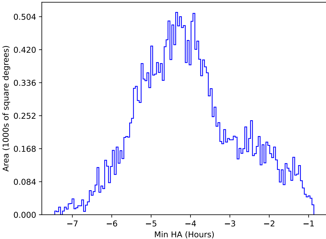
roll_pause_mjdp60_v3.4_10yrs All sky z band: Min HA
