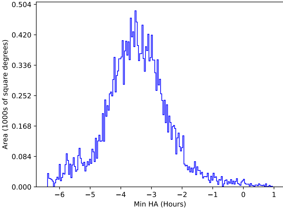
roll_pause_mjdp60_v3.4_10yrs All sky y band: Min HA
