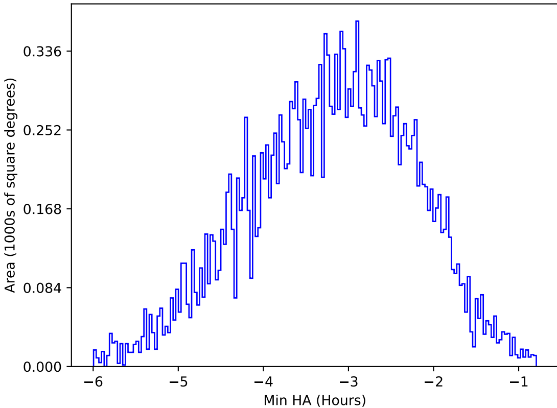
roll_pause_mjdp60_v3.4_10yrs All sky u band: Min HA
