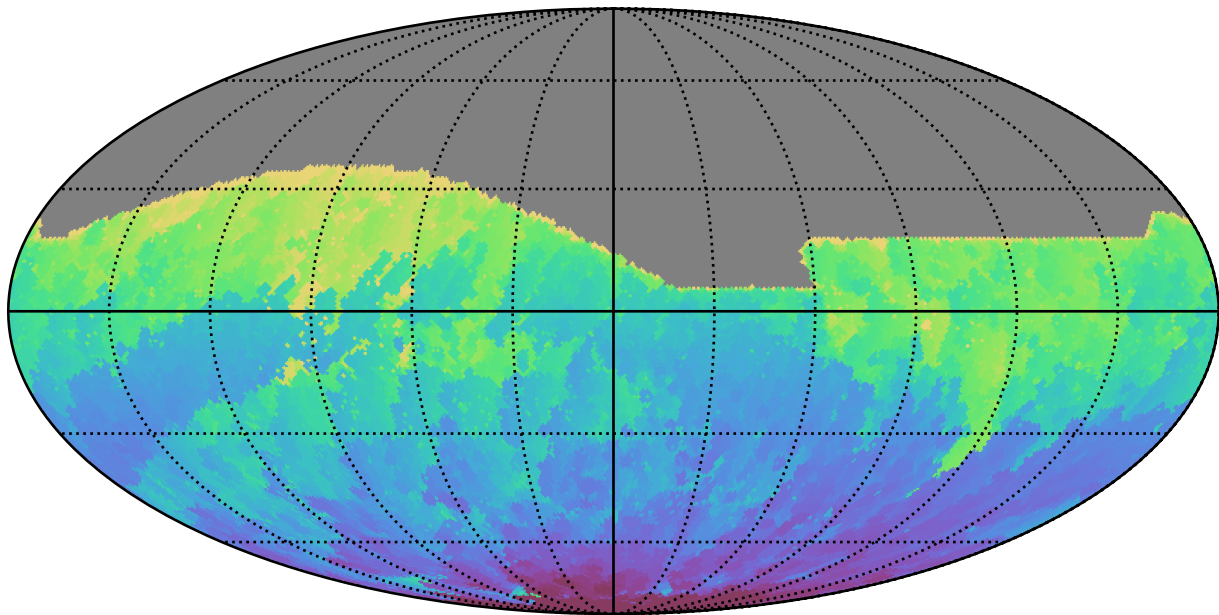
roll_pause_mjdp60_v3.4_10yrs All sky i band: Min HA
