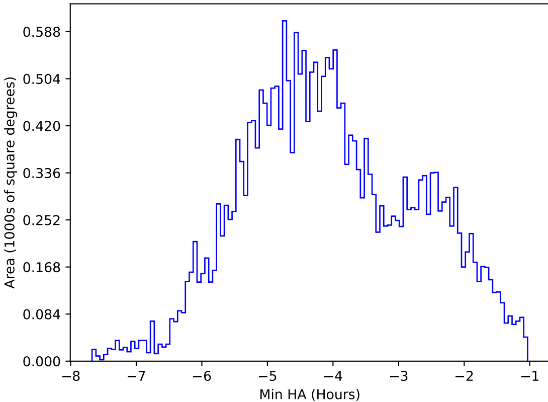
roll_pause_mjdp60_v3.4_10yrs All sky i band: Min HA
