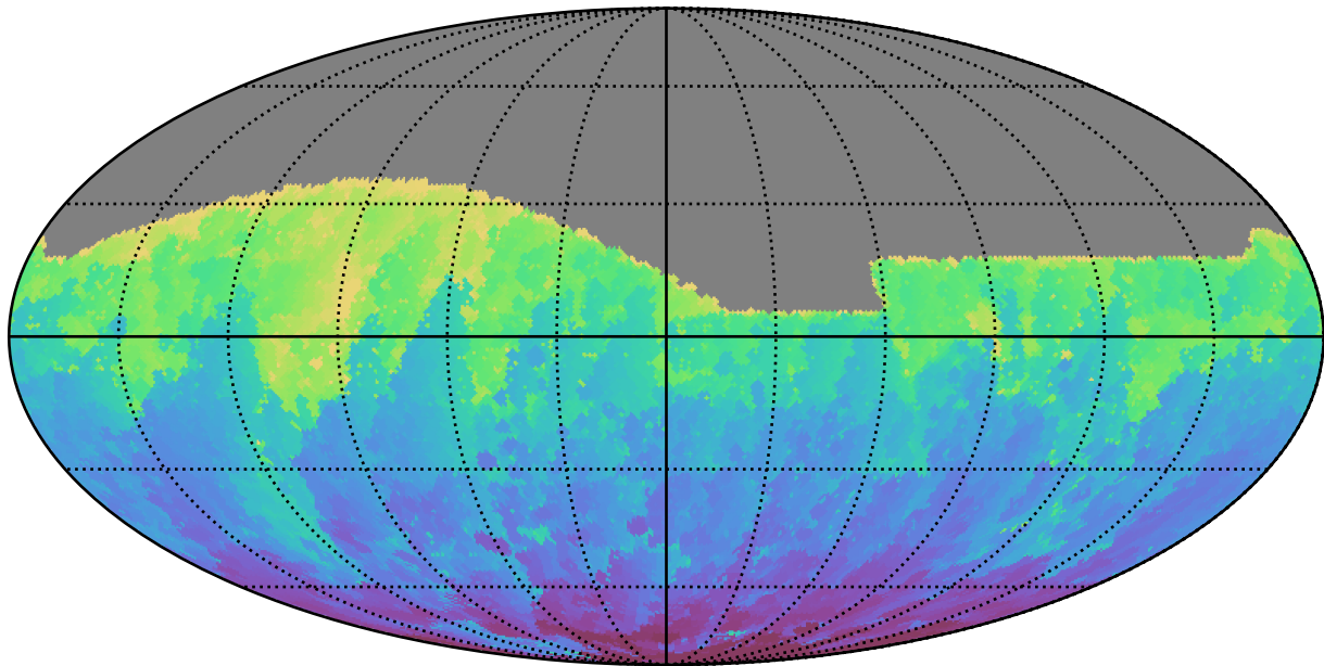
roll_pause_mjdp60_v3.4_10yrs All sky g band: Min HA
