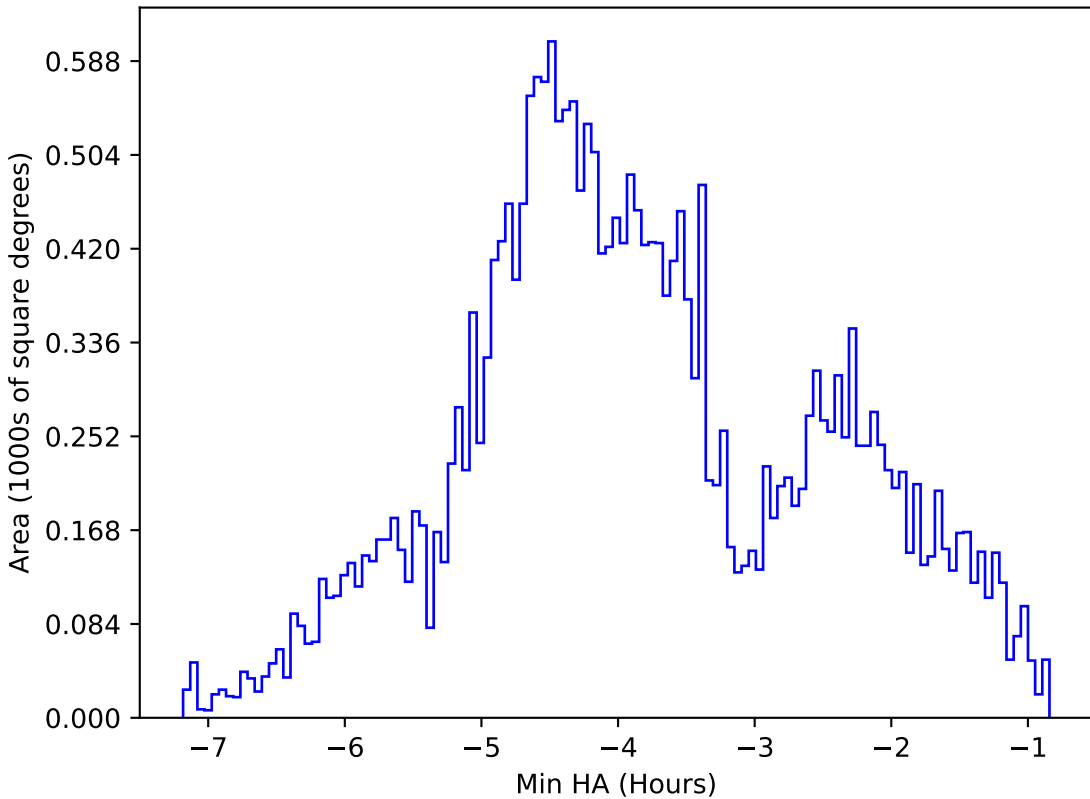
roll_pause_mjdp60_v3.4_10yrs All sky g band: Min HA
