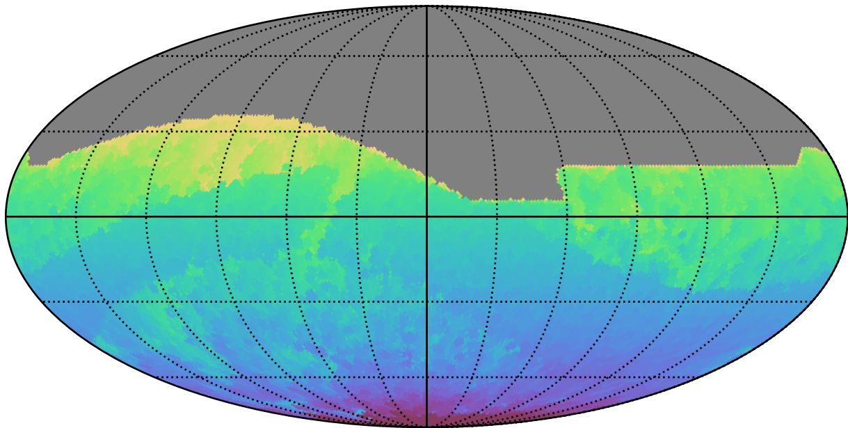
roll_pause_mjdp60_v3.4_10yrs All sky all bands: Min HA
