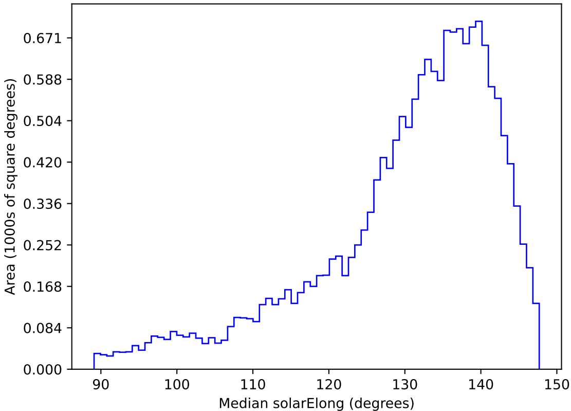
roll_pause_mjdp60_v3.4_10yrs WFD y band: Median solarElong
