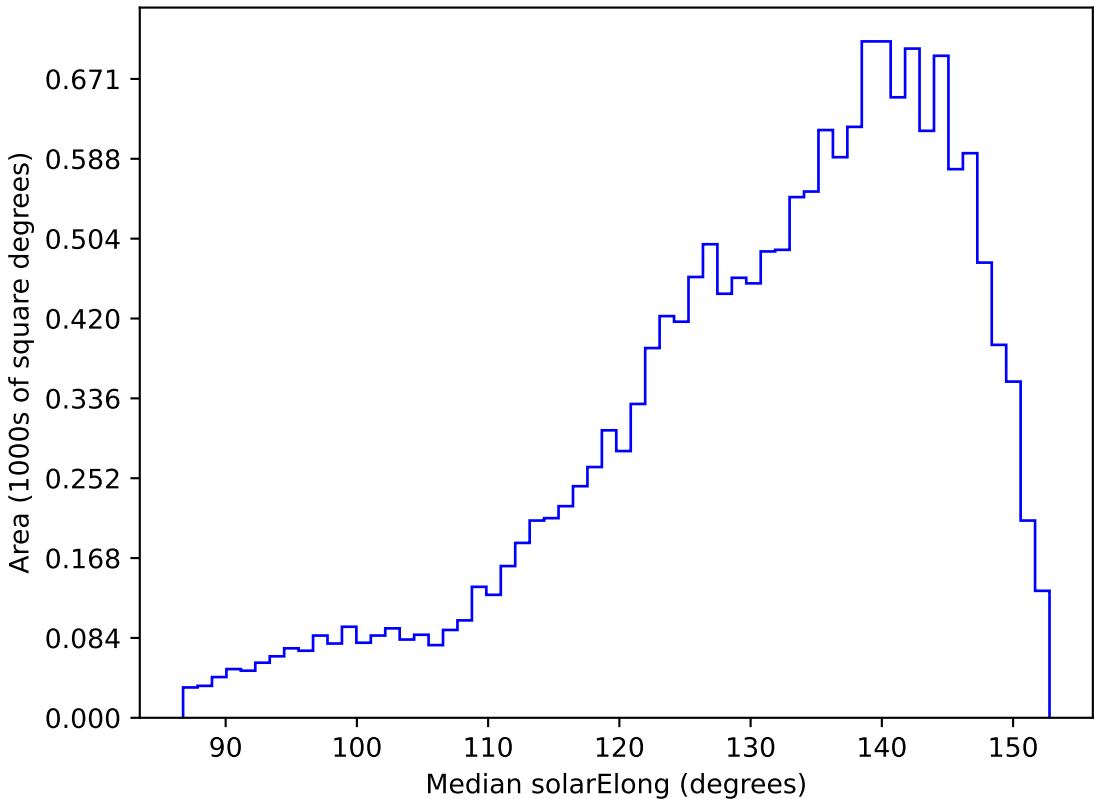
roll_pause_mjdp60_v3.4_10yrs WFD u band: Median solarElong
