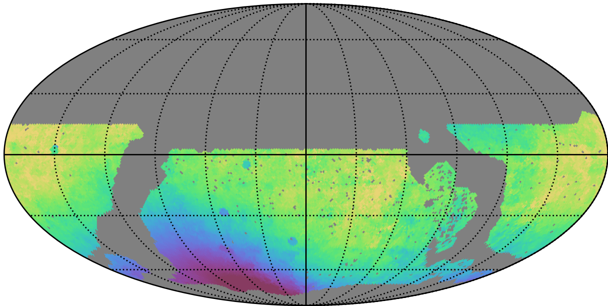
roll_pause_mjdp60_v3.4_10yrs WFD r band: Median solarElong
