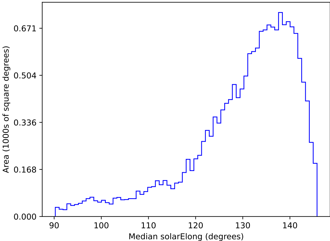
roll_pause_mjdp60_v3.4_10yrs WFD r band: Median solarElong
