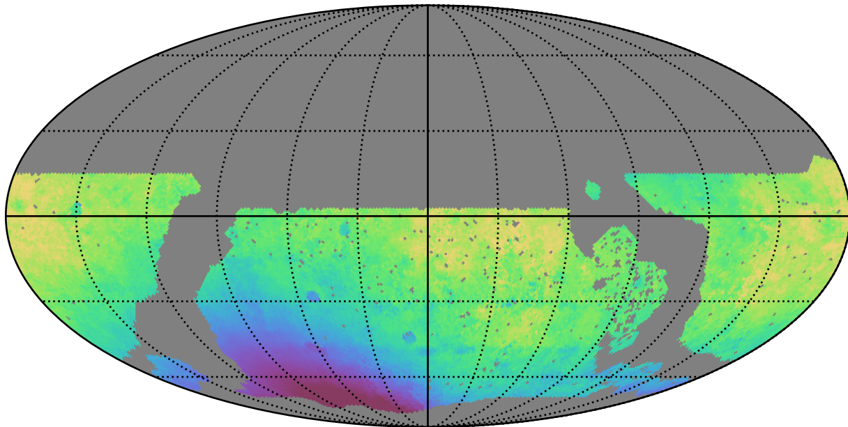
roll_pause_mjdp60_v3.4_10yrs WFD i band: Median solarElong
