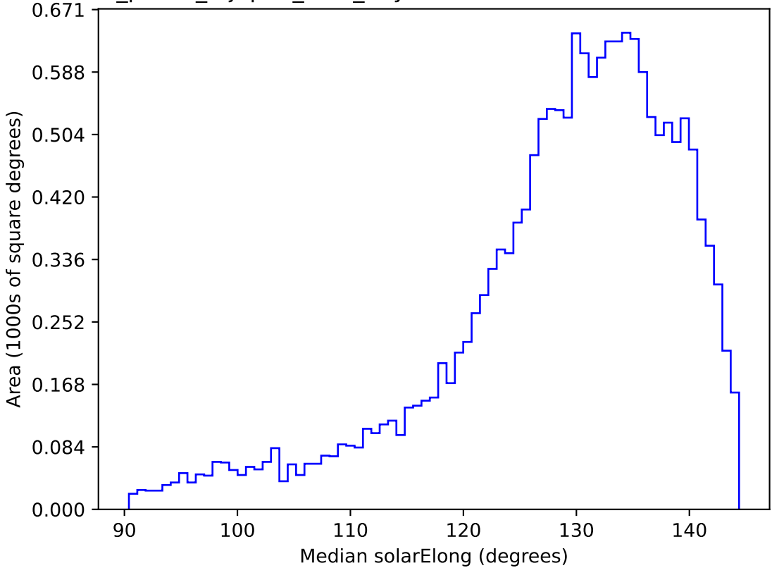
roll_pause_mjdp60_v3.4_10yrs WFD i band: Median solarElong
