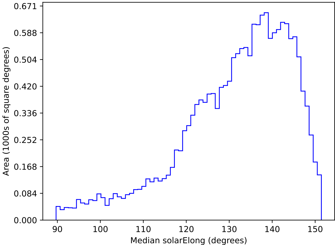
roll_pause_mjdp60_v3.4_10yrs WFD g band: Median solarElong
