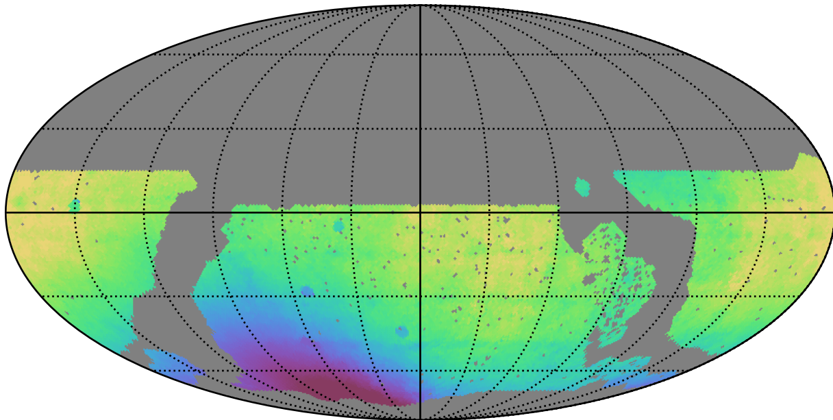
roll_pause_mjdp60_v3.4_10yrs WFD all bands: Median solarElong
