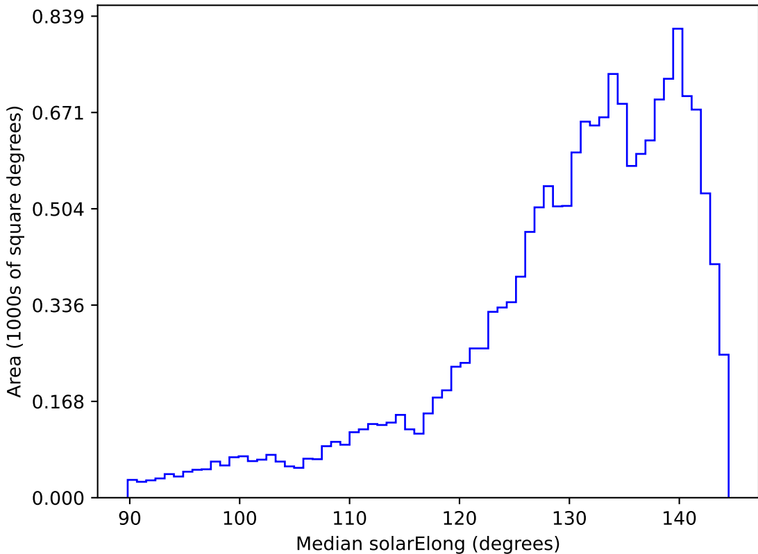
roll_pause_mjdp60_v3.4_10yrs WFD all bands: Median solarElong
