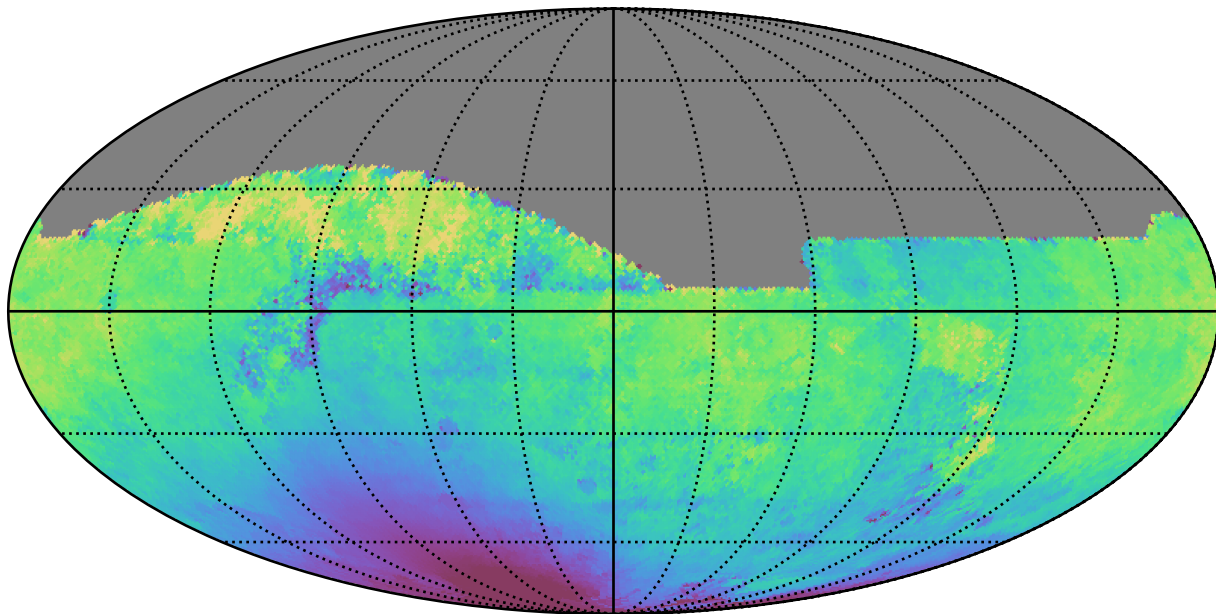
roll_pause_mjdp60_v3.4_10yrs All sky z band: Median solarElong
