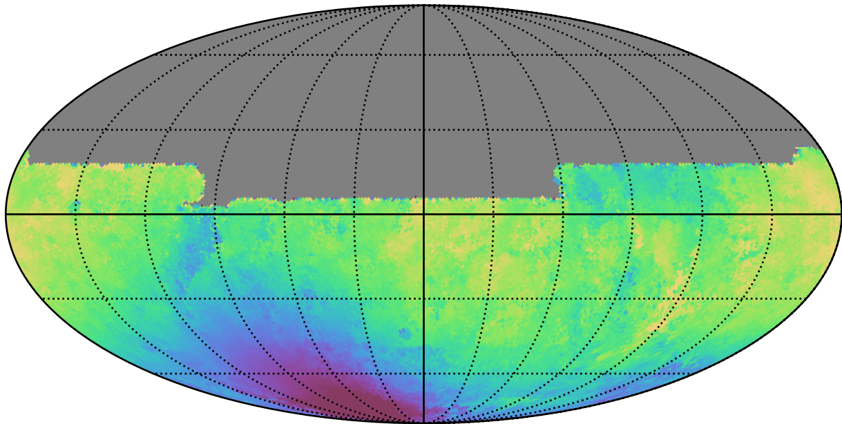
roll_pause_mjdp60_v3.4_10yrs All sky y band: Median solarElong
