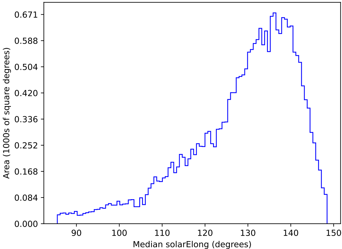
roll_pause_mjdp60_v3.4_10yrs All sky y band: Median solarElong
