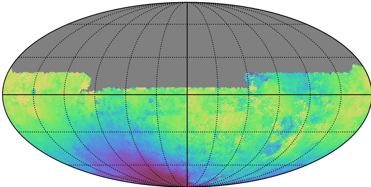
roll_pause_mjdp60_v3.4_10yrs All sky u band: Median solarElong
