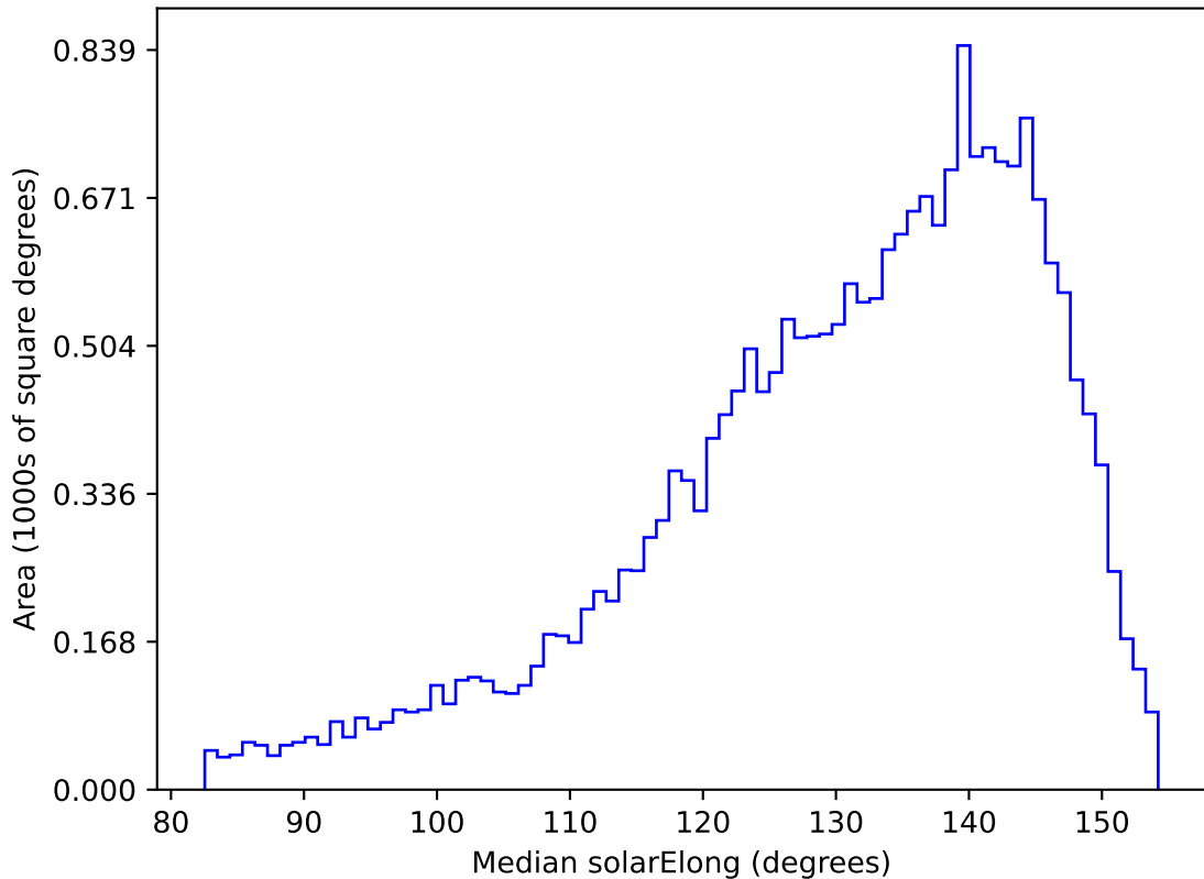
roll_pause_mjdp60_v3.4_10yrs All sky u band: Median solarElong
