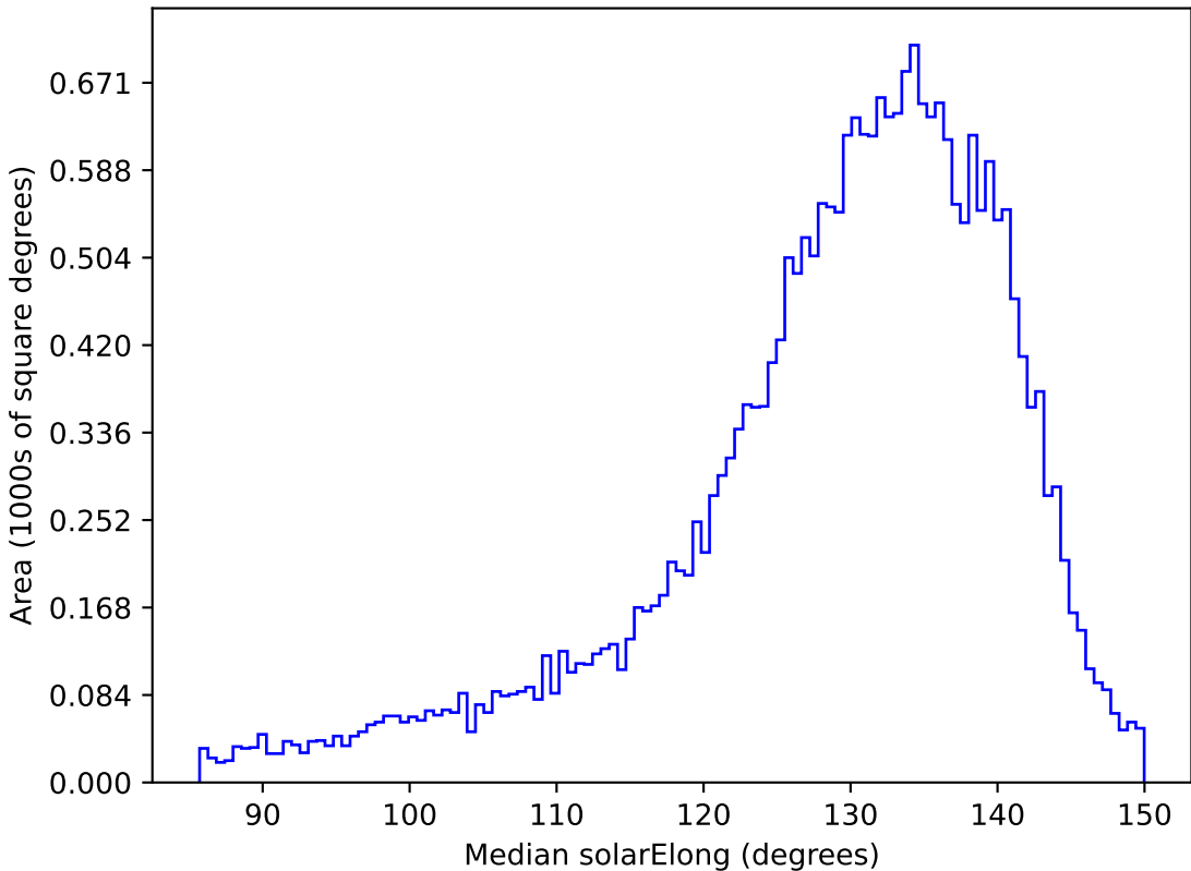
roll_pause_mjdp60_v3.4_10yrs All sky i band: Median solarElong
