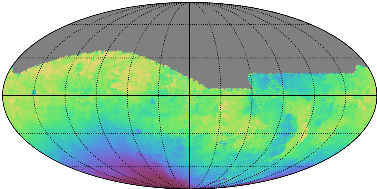
roll_pause_mjdp60_v3.4_10yrs All sky g band: Median solarElong
