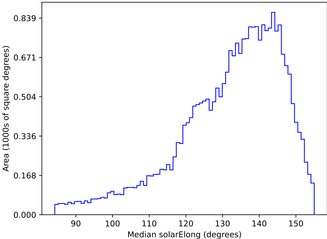
roll_pause_mjdp60_v3.4_10yrs All sky g band: Median solarElong
