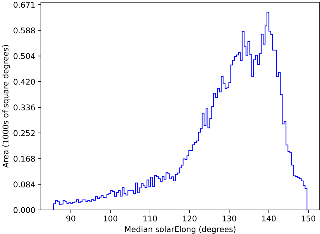
roll_pause_mjdp60_v3.4_10yrs All sky all bands: Median solarElong
