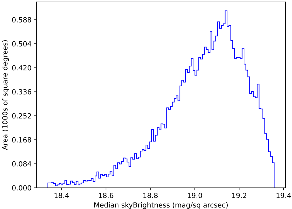
roll_pause_mjdp60_v3.4_10yrs Yr 1 z band: Median skyBrightness
