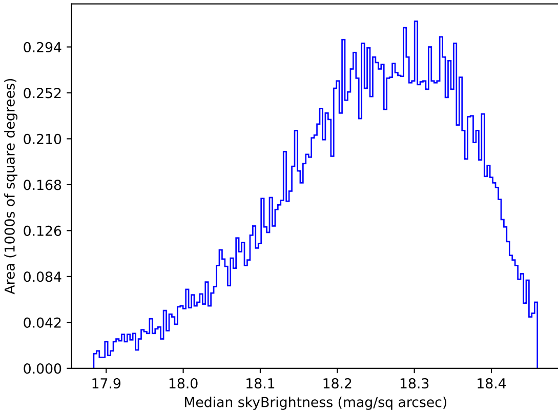
roll_pause_mjdp60_v3.4_10yrs Yr 1 y band: Median skyBrightness
