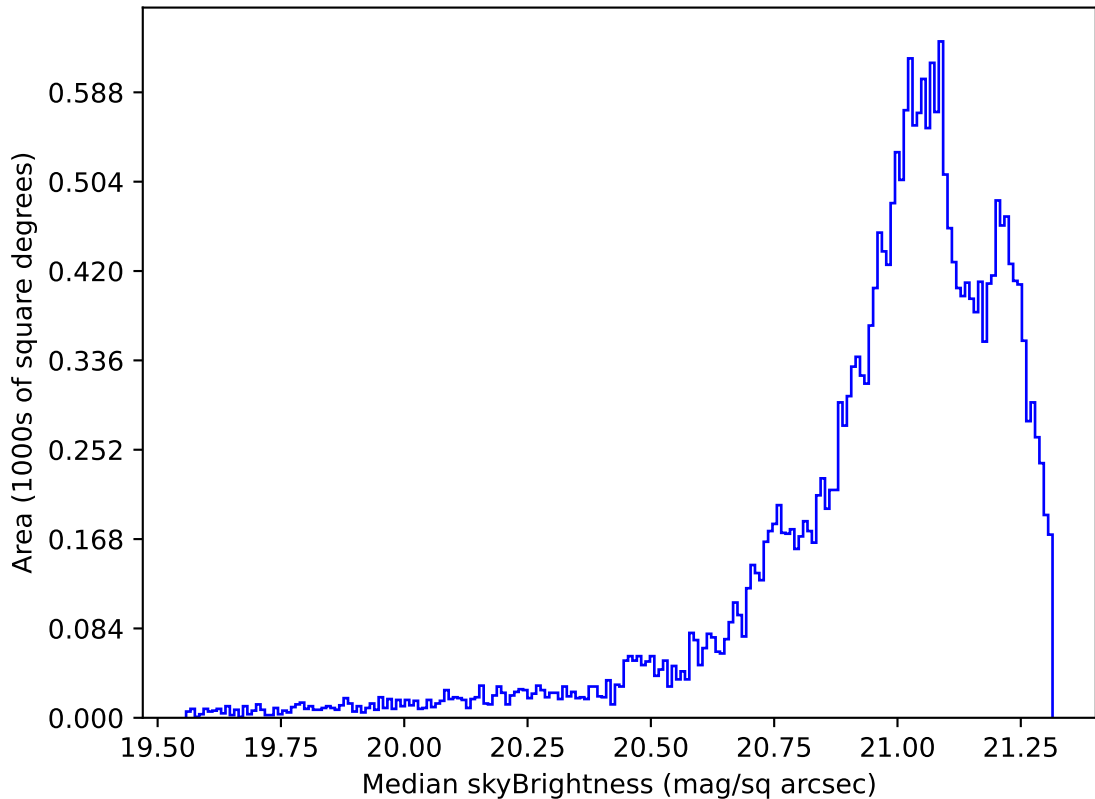
roll_pause_mjdp60_v3.4_10yrs Yr 1 r band: Median skyBrightness
