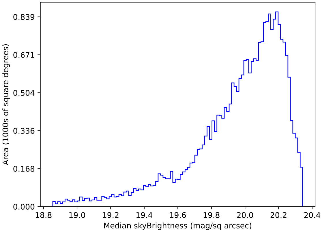
roll_pause_mjdp60_v3.4_10yrs Yr 1 i band: Median skyBrightness
