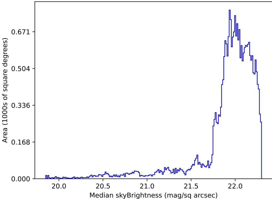
roll_pause_mjdp60_v3.4_10yrs Yr 1 g band: Median skyBrightness
