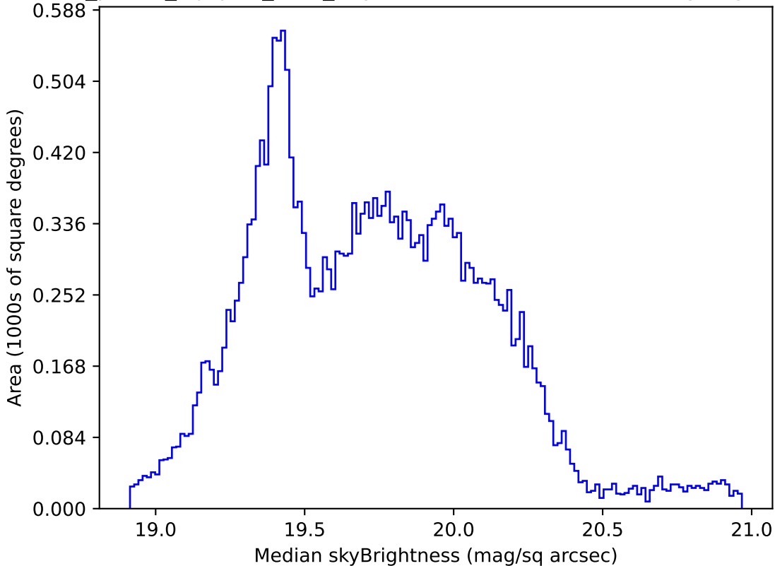
roll_pause_mjdp60_v3.4_10yrs Yr 1 all bands: Median skyBrightness
