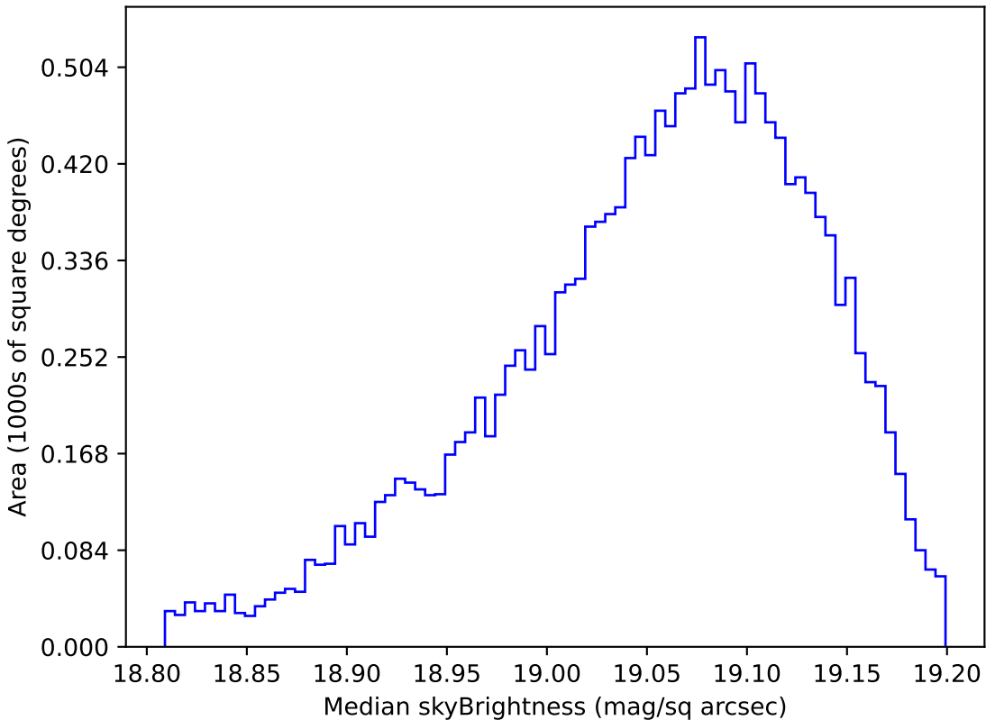
roll_pause_mjdp60_v3.4_10yrs WFD z band: Median skyBrightness
